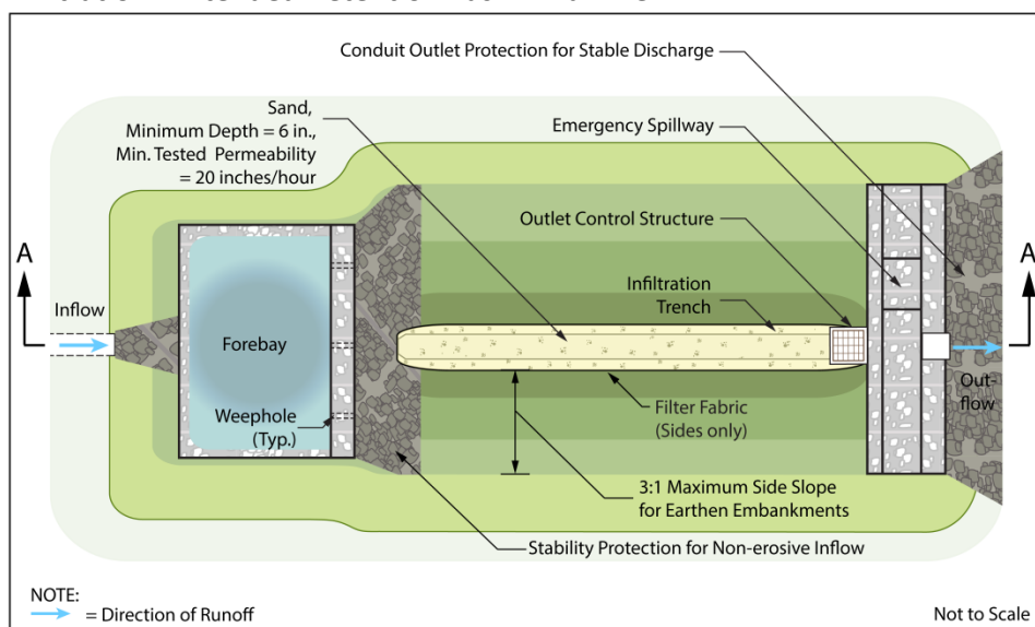
Infiltration - Extended Detention Basin: Plan View
